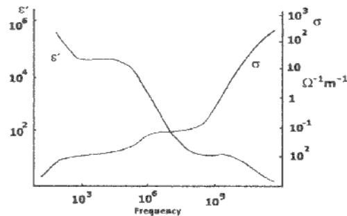
Fig.1 – Variation of \epsilon' (dielectric constant) and conductivity \sigma of high water content tissue as a function of non ionizing radiation.
