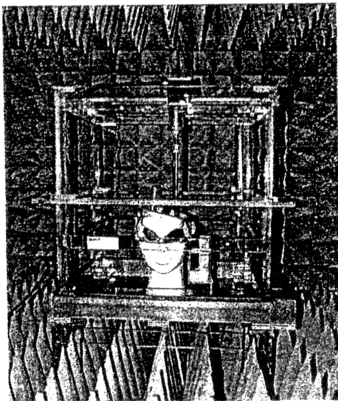
Figure 1: Arrangement for SAR-measurements in a heterogeneous phantom with support frame (left) and head and hand phantom with a phone (right)
