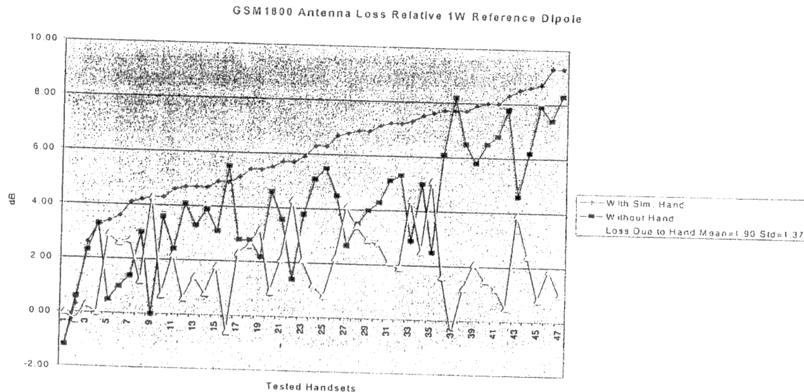
Figure 5. GSM1800 handset antenna loss, including phantom and with/without simulated hand, relative to 60° tilted dipole. Extractable antennas are extracted. Median values are 6.30 dB and 3.90 dB. Mean loss due to simulated hand is 1.90 dB with a standard deviation of 1.37 dB.
