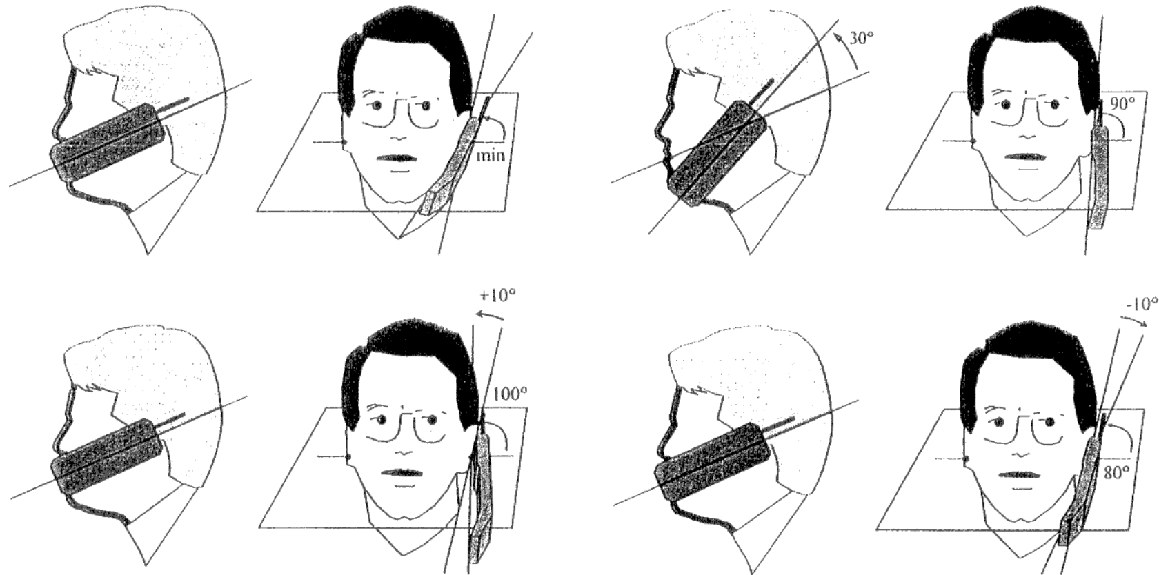
Figure 1: Test positions for SAR measurements. Touch (top left), 30° (top right), 100° (below left) and intended use position (below right).
