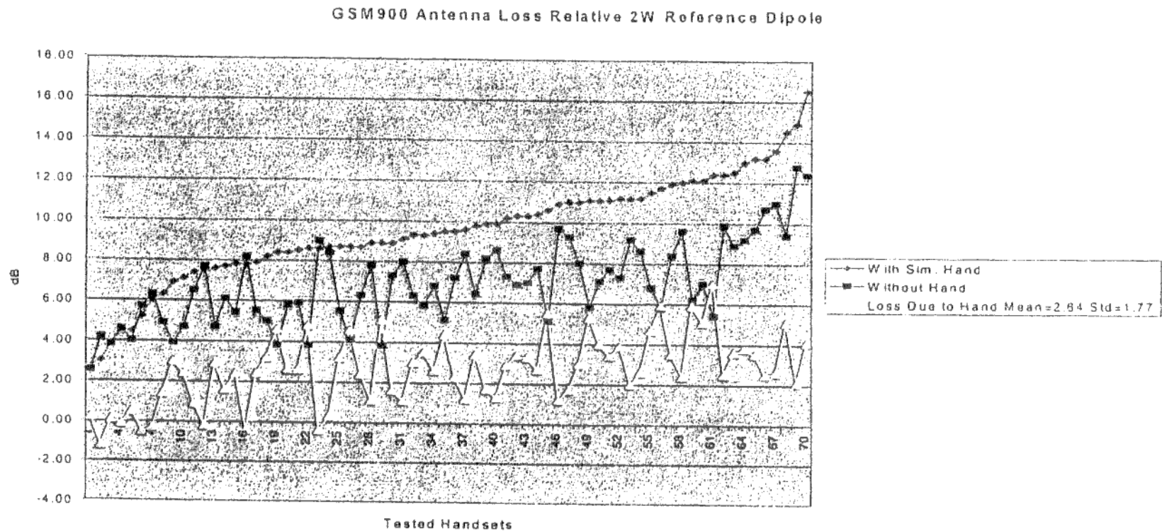
Figure 4. GSM900 handset antenna loss, including phantom and with/without simulated hand, relative to 60° tilted dipole. Extractable antennas are extracted. Median values are 9.50 dB and 6.85 dB. Mean loss due to simulated hand is 2.64 dB with a standard deviation of 1.77 dB.
