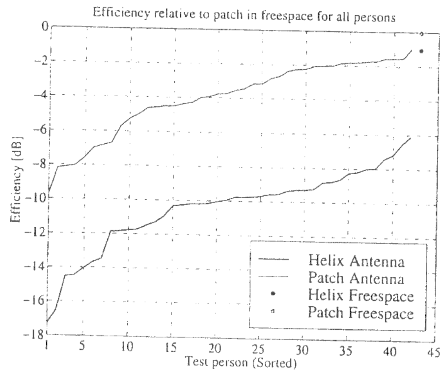
Figure 5: Transmitted power by the mobile phone held by 43 different persons measured in an anechoic room.
